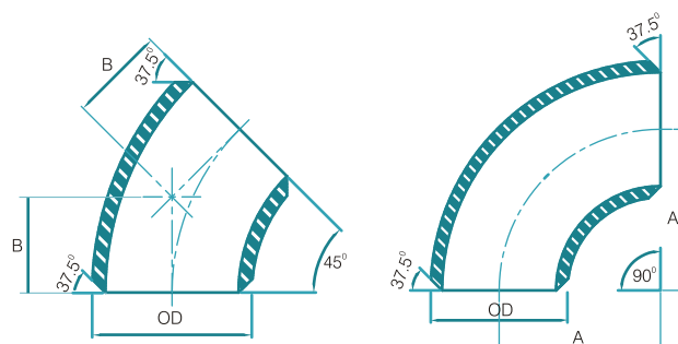
SEAMLESS ELBOW
