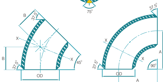
WELDED ELBOW
